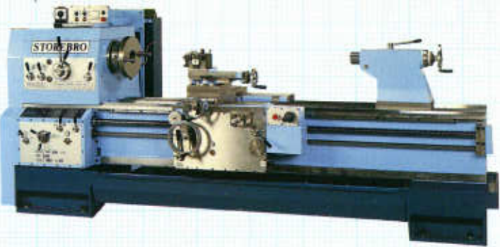
STOREBRO SB 255/305/355 -N centre height/distance 255, 305, 355/1500-6000 mm spindle bore up to 310 mm
